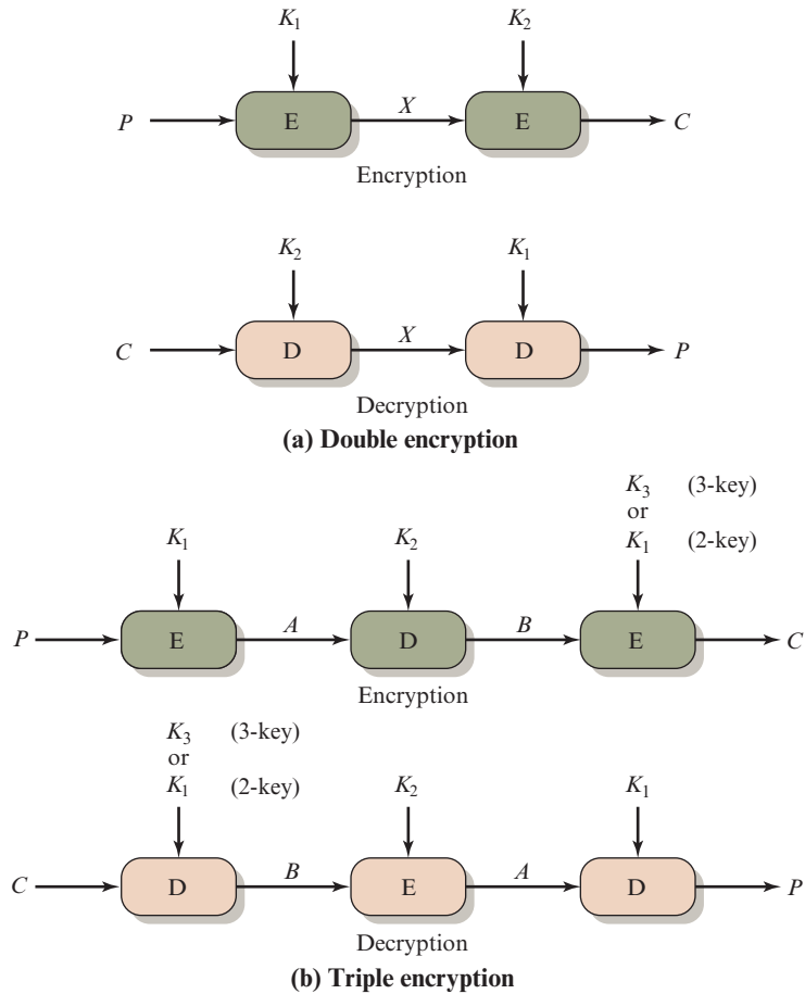
Figure 7.1 Multiple Encryption
