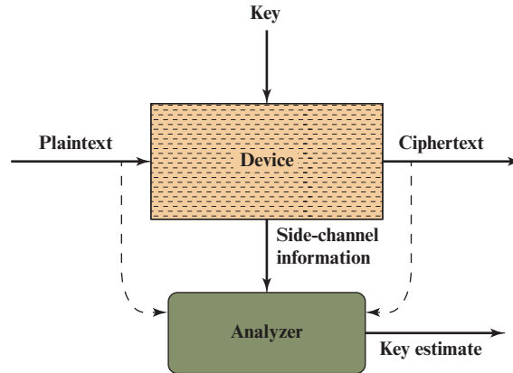
Figure 14.3 Side-Channel Attack
