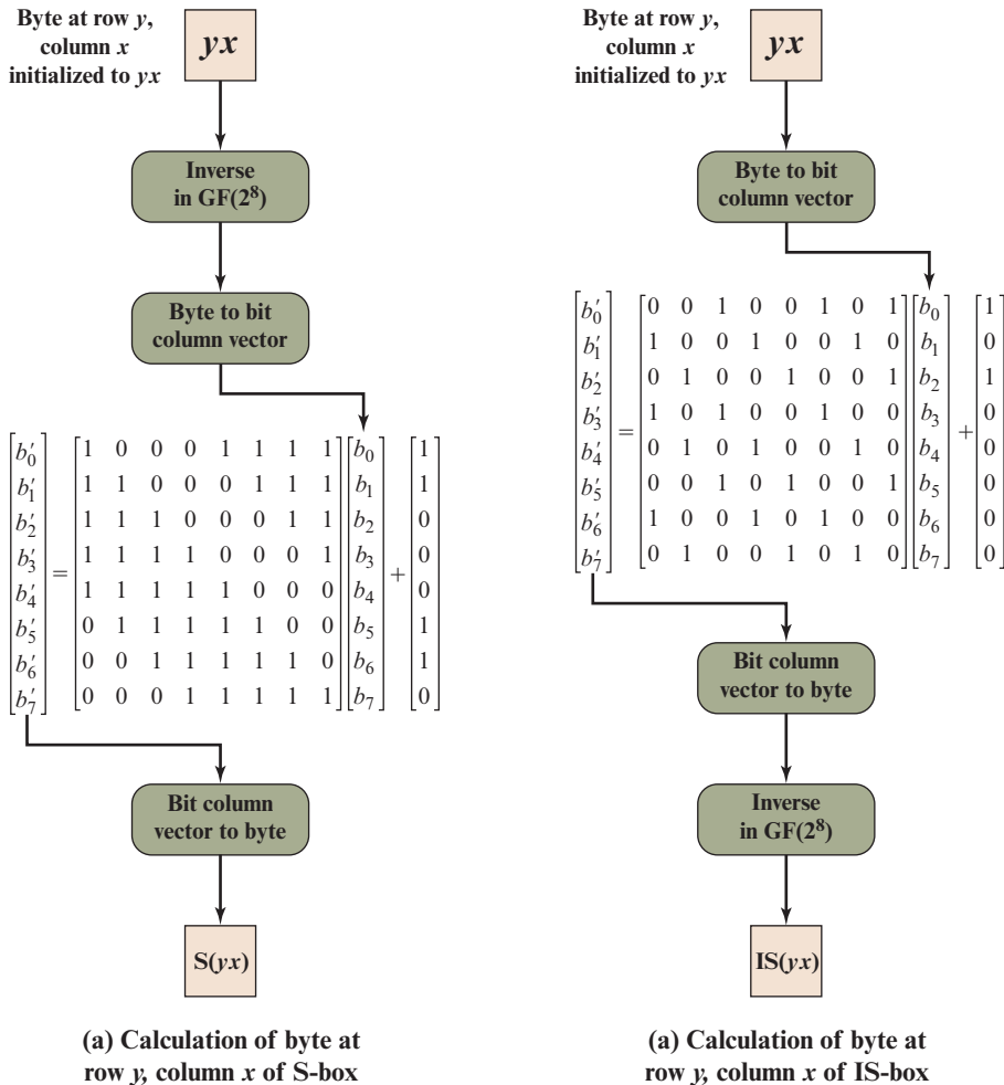
Figure 6.6 Construction of S-Box and IS-Box
