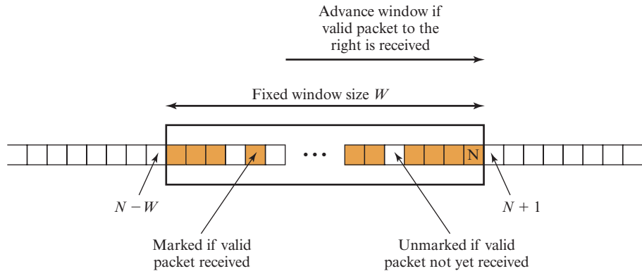
Figure 20.5 Anti-replay Mechanism
