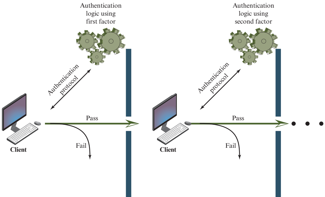
Figure 16.2 Multifactor Authentication
