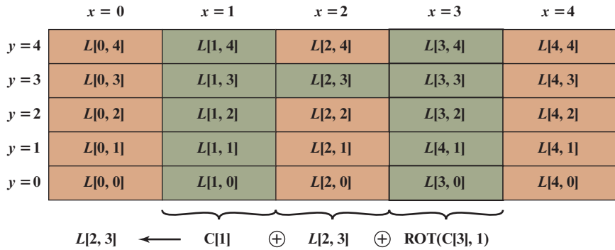
(a) \theta step function
